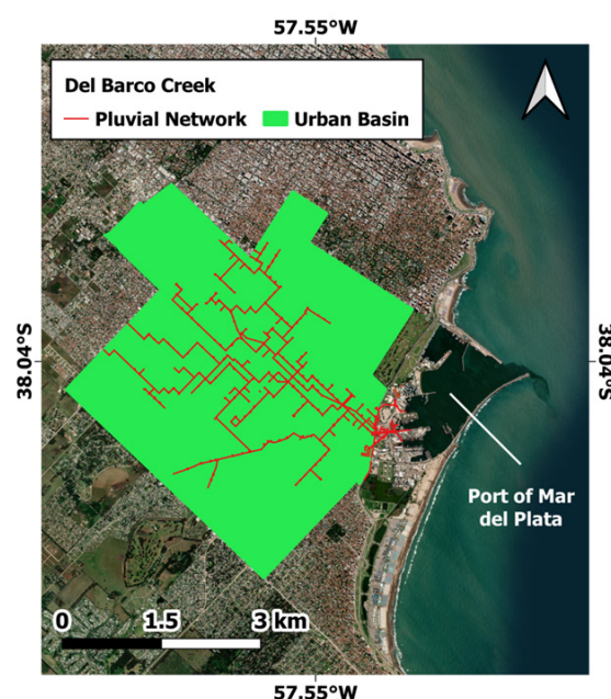
Figure 9. Del Barco creek urban basin and its pluvial network. It supports 14 neighborhoods in the southern area of Mar del Plata, discharging in the port. Source: open access database of the General Pueyrredon County ( https://datos.mardelplata.gob.ar/ )
